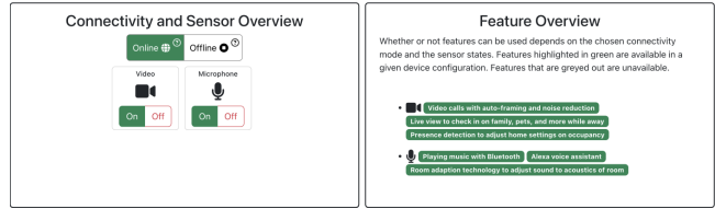
Figure 8: The interactive privacy label we used in the survey for the Amazon Echo Show 8. The features and sensors were extracted from the manufacturer’s official product pages.
