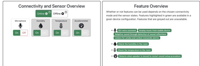
Figure 9: The interactive privacy label we used in the survey for the Apple HomePod. The features and sensors were extracted from the manufacturer’s official product pages.
