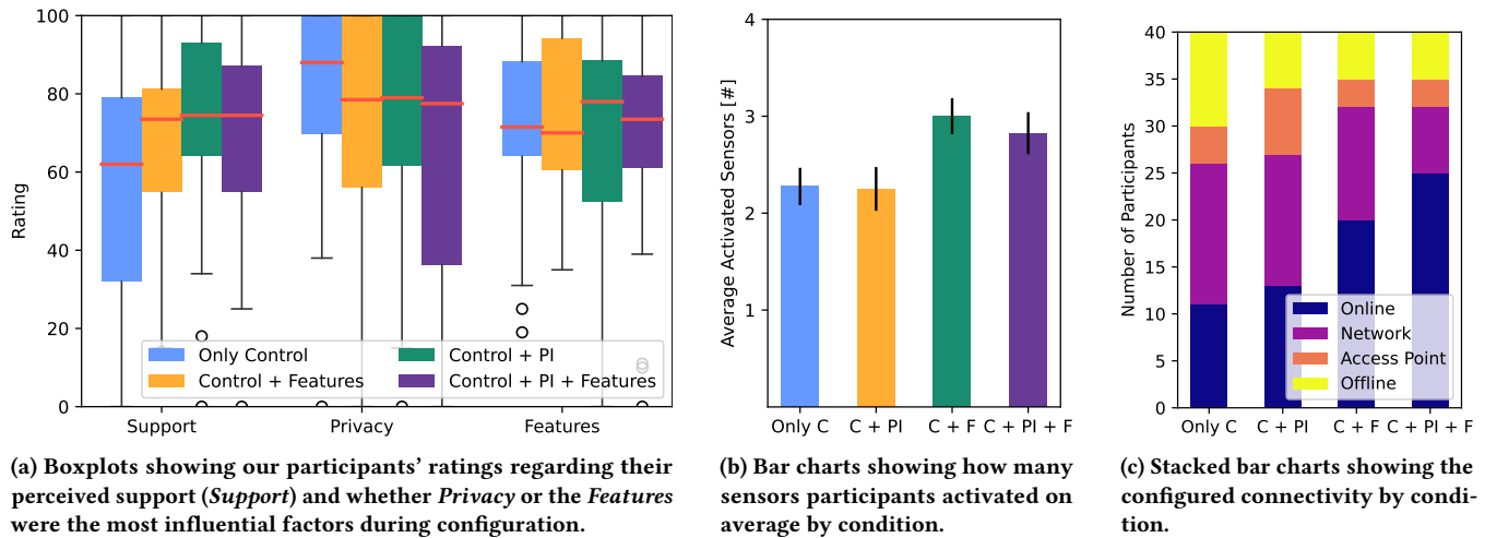
Figure 6: Visualization of the results from task 1. PI refers to conditions in which the Privacy Index was shown.
