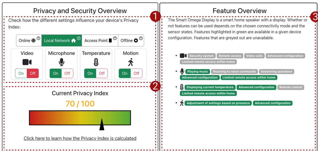
Figure 1: The final interactive smart device privacy label, based on an iterative design process with in-depth feedback from expert interviews. The boxes mark the label’s key components: (1) the control component that enables users to change the connectivity mode (top) and the state of individual sensors (bottom); (2) the privacy index that reflects the privacy exposure based on the configuration from (1); and (3) a feature overview that dynamically reflects the available feature set based on the configuration (1).
